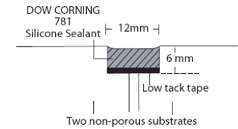
Figure 2: Shallow joint.
